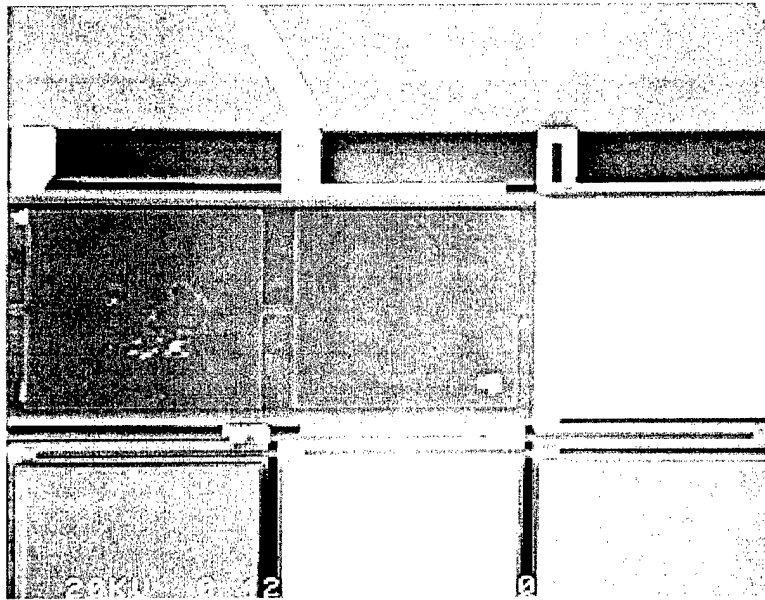
Figure 3-6. SEM photo of MUMPs™ LAMA elements with top mirror plates removed. Photo orientation shows rows connected in the vertical direction, with POLY 0 columns connected across horizontally underneath. Note rows are connected from opposite sides of the package in an alternating fashion.
